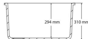
Side cross-section
